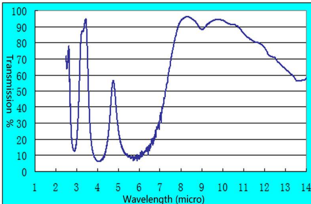
Transmission of Si windows with AR@8-12 micro
